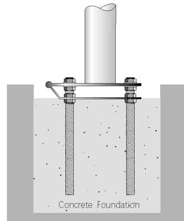
FIG 2. BASEPLATE FOUNDATION
