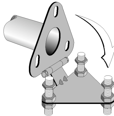
FIG 1. BASEPLATE
